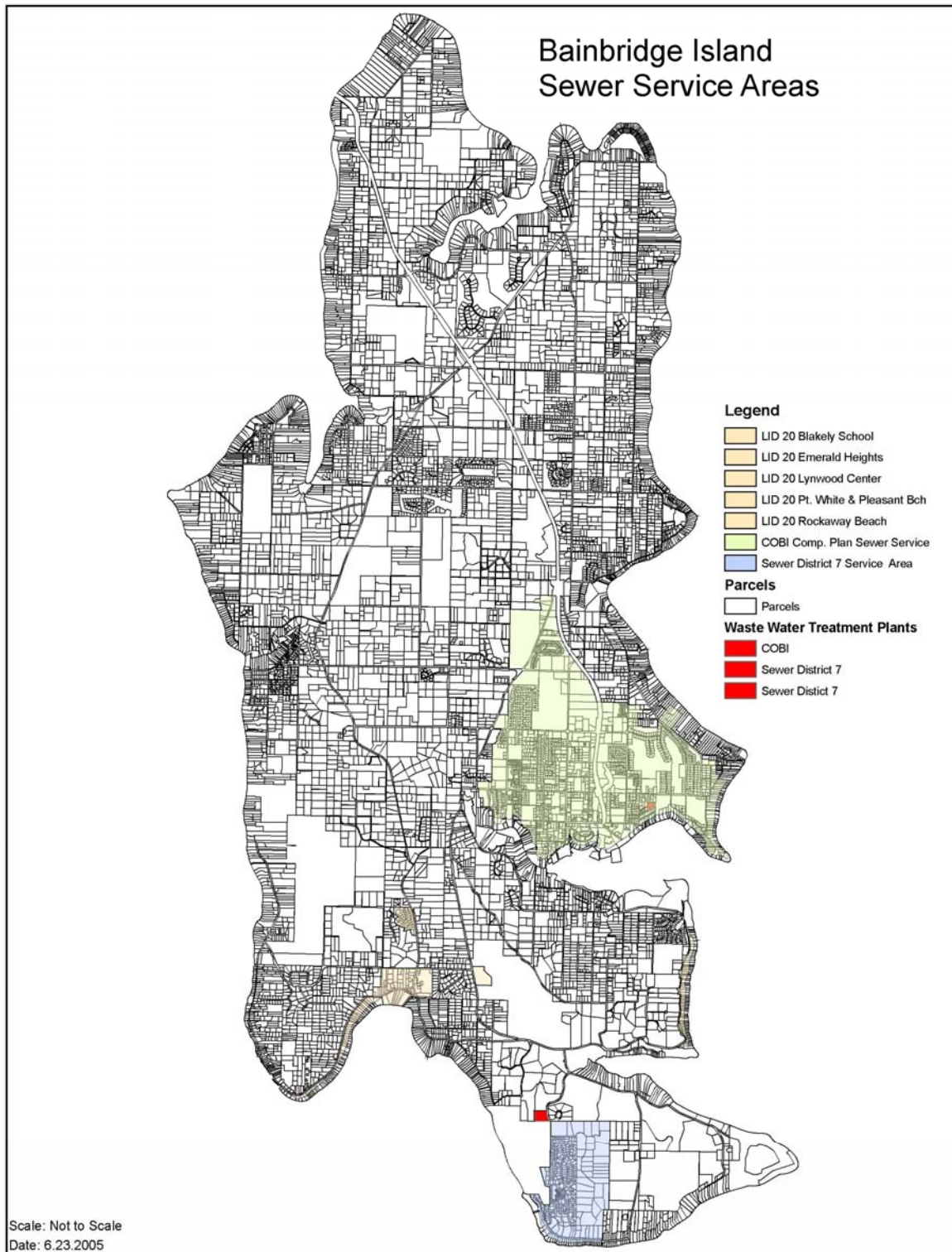
Figure 1: Bainbridge Island Sewer Service Area
